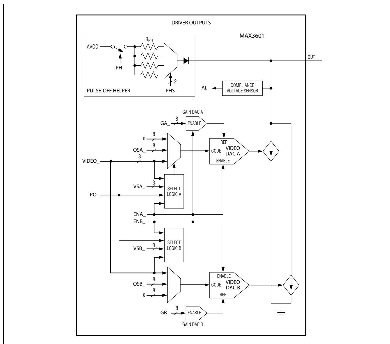
Figure 10. Driver Output
